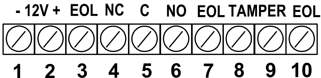
Fig.3. Wiring connections
